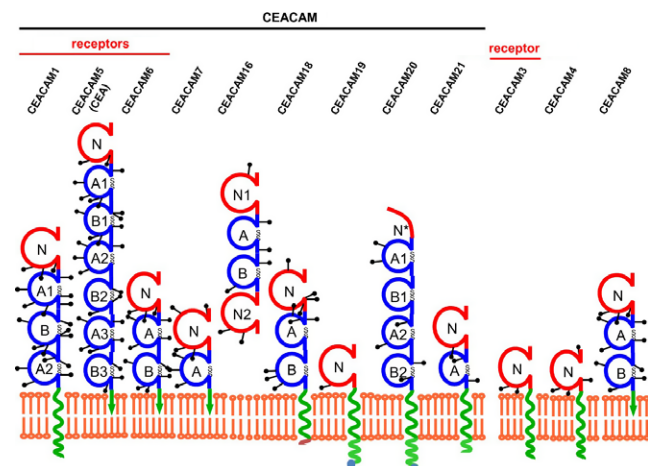
FIGURE 1 The carcinoembryonic antigen-related cell adhesion molecule (CEACAM) gene superfamily. 79 The CEACAM immunoglobulin-like domain superfamily is a large family of proteins encoded by 12 independent genes and located on chromosome 19. The Ig domain consists generally of one IgV-like N-domain (red), except CEACAM 16, which has 2 N-domains and IgC-like domains identified as (A and B) shown in (blue). The membrane-linked glycoproteins are anchored to the cell surface either by transmembrane domain (green zigzag lines), such as CEACAM5-8, or anchored to the membrane by glycoposphatidyl-inositol anchor (green arrowhead), including CEACAM1, 3, 4, 19, 20 and 21. CEACAM16 is a secreted version with no membrane anchorage. The CEACAM 19 and 20 cytoplasmic domain has immune-receptor tyrosine-based activator (ITAM) motifs (blue circles). Heavily N-Glycosylation sites in all family members are shown as black lippops on the extracellular domains
