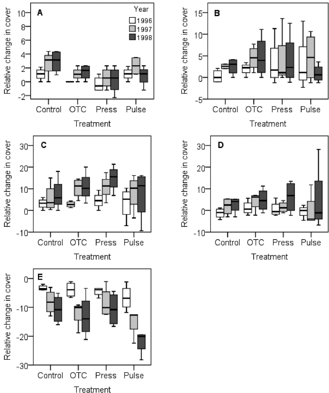
Figure 3. Boxplots of responses in relative change in cover in plant functional groups in the alpine meadow. (A) Cushions, (B) deciduous shrubs, (C) evergreens, (D) forbs, and (E) graminoids. Treatments: control (Control), constant warming enhancement using open-top chambers (OTC), a stepwise increase in the magnitude of warming (Press) and a single-summer high-impact warming event (Pulse). Boxplots show the 10 th to 90 th percentiles of the data; n = 4 plots per treatment.
